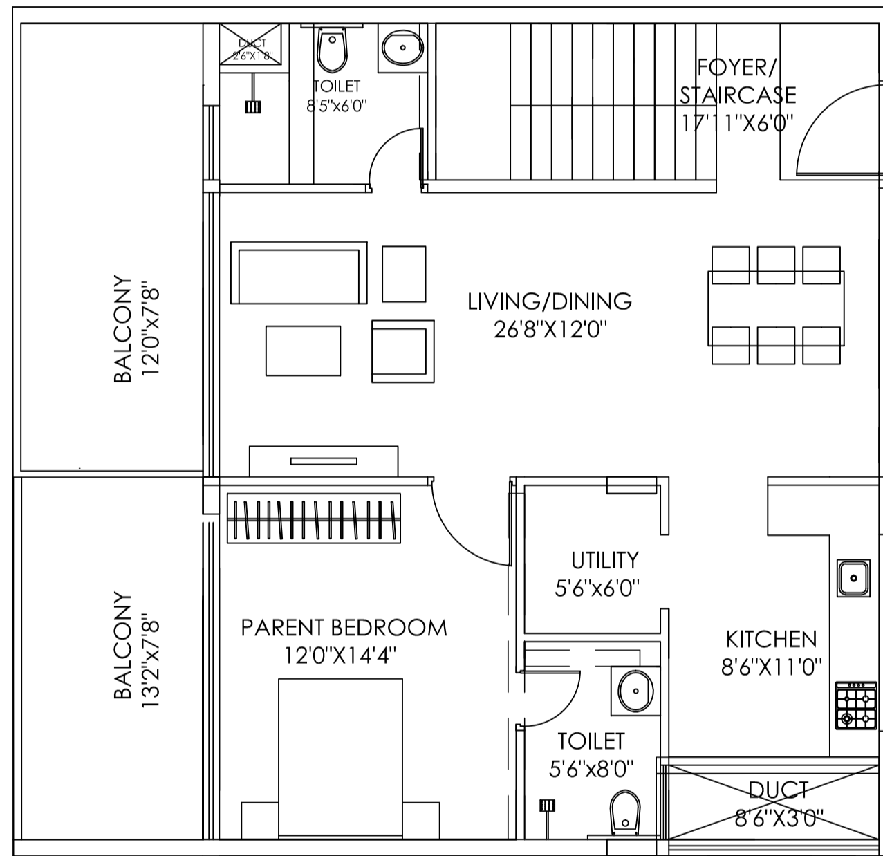
SECOND FLOOR PLAN 1225 SFT
