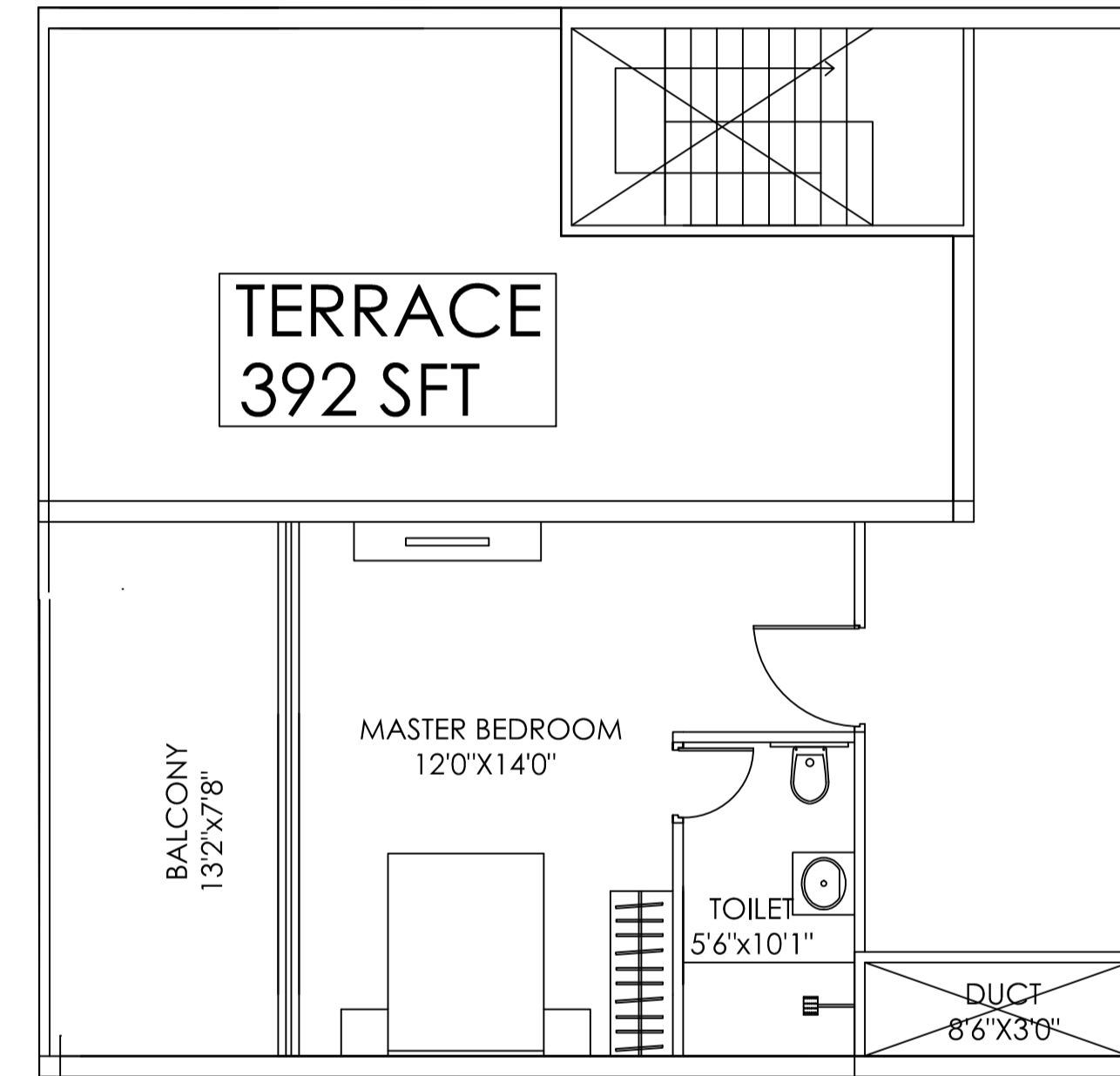
TERRACE FLOOR PLAN 852 SFT
